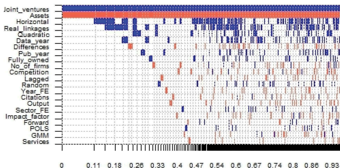
Figure 3. Model inclusion in Bayesian model averaging.
