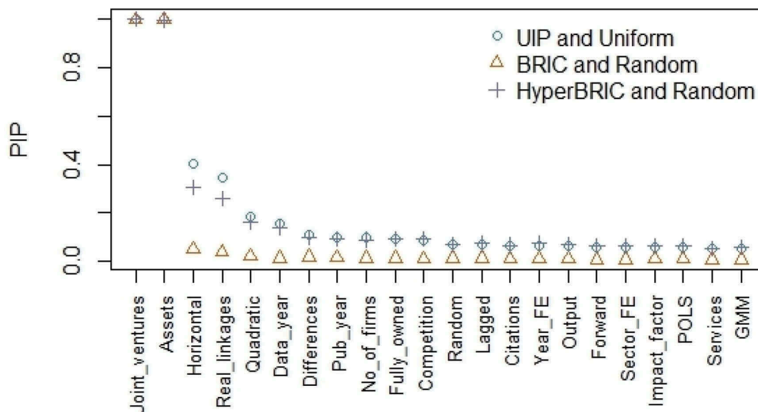
Figure 4. Posterior inclusion probabilities across different prior settings.
